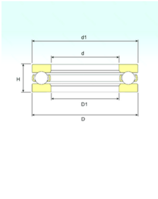
51109 Bearing 2D drawings and 3D CAD models
