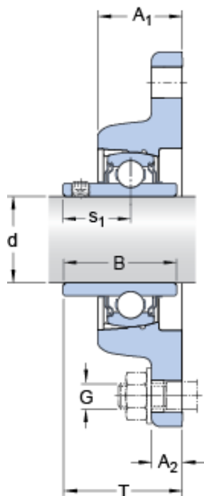
FYT 2. TF/VA201 Bearing 2D drawings and 3D CAD models
